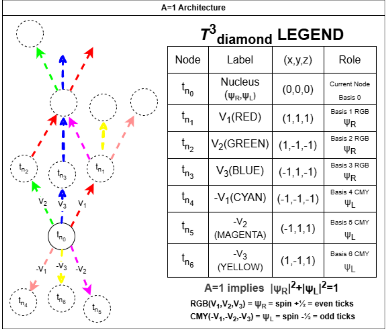
Figure 1: The \mathcal{T}_\diamond^3 lattice architecture. The nucleus node t_{n_0} carries both Dirac spinor components ( \psi_R, \psi_L ). RGB basis vectors constitute the right-handed sublattice ( \psi_R , spin +1/2 , even ticks) and CMY basis vectors the left-handed sublattice ( \psi_L , spin -1/2 , odd ticks). The A=1 constraint requires |\psi_R|^2 + |\psi_L|^2 = 1 .
