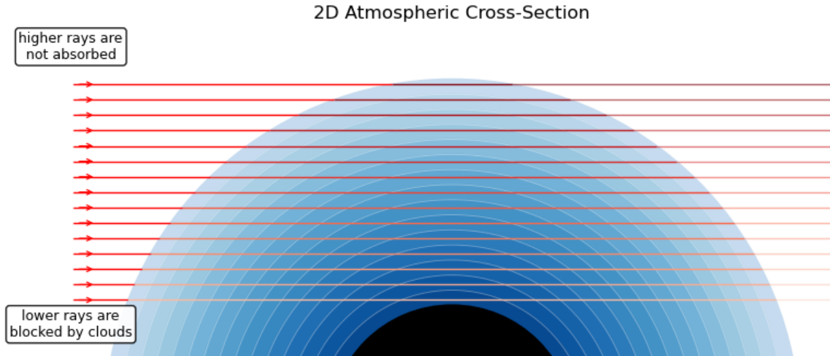
Figure 1: Diagram illustrating the radiative transfer process in an exoplanet atmosphere.
