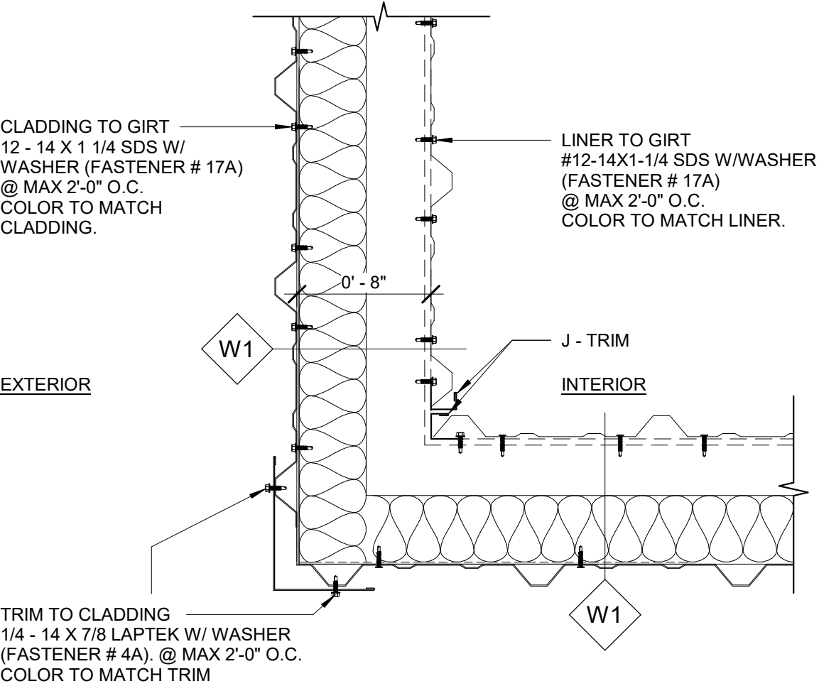
3 FASTENER SPACING DETAIL GA-450 1 1/2" = 1'-0"
