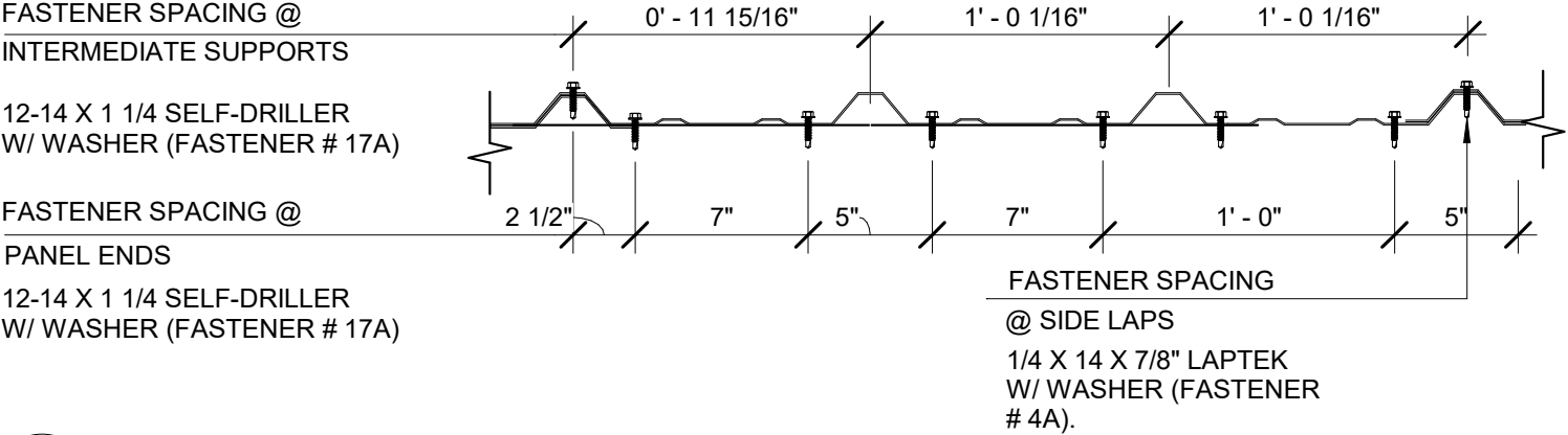
3 FASTENER SPACING DETAIL GA-450 1 1/2" = 1'-0"
