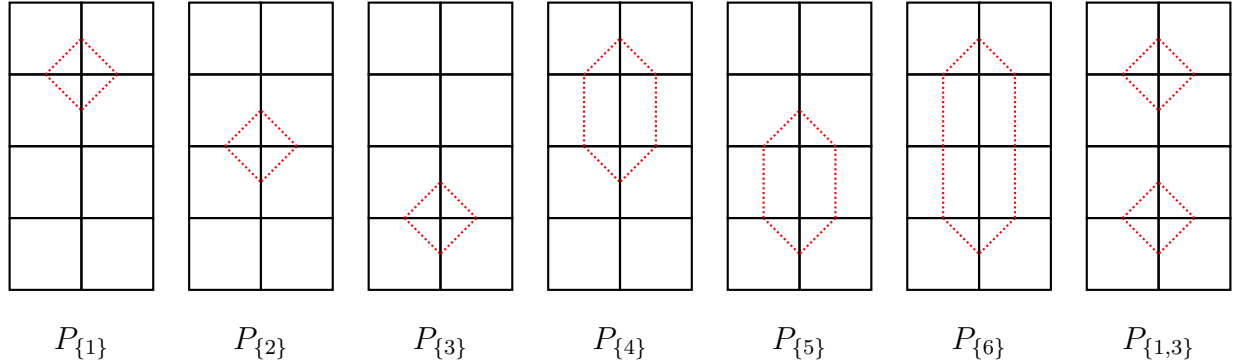
Figure 8: All (4, 2) polygon mosaics except P_\emptyset
