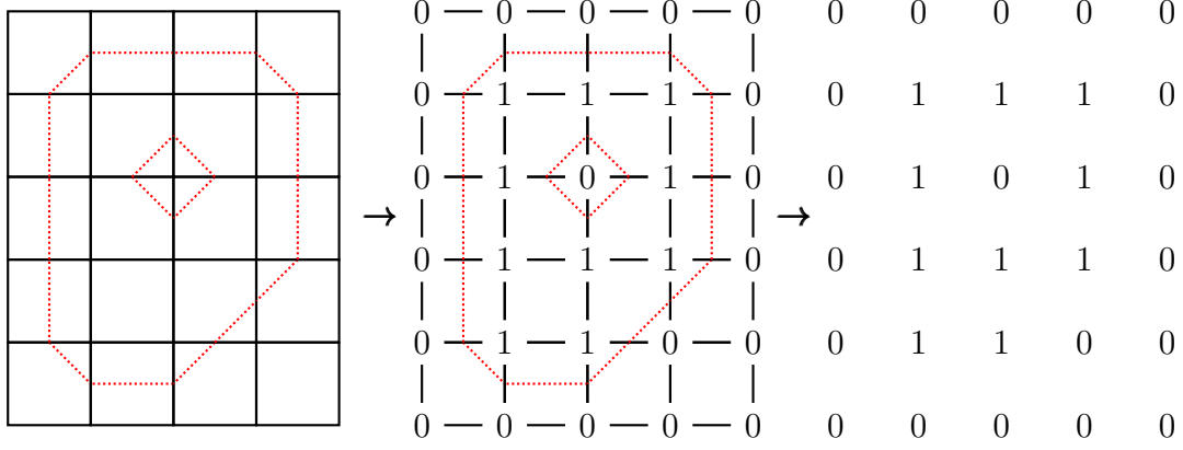
Figure 3: Applying \mathcal{L} to a polygon mosaic
