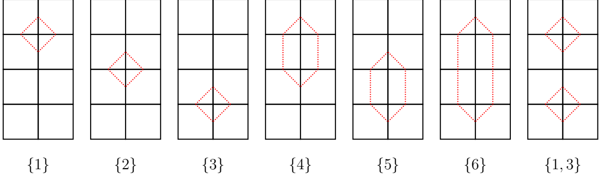
Figure 7: (4, 2) polygon mosaics with names
