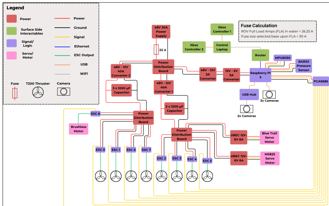
Figure 2. System interconnect diagram, 2026 vehicle, drawn by the author. Red: power; black: ground; yellow: signal; blue: Ethernet; green: ESC output. Full-load current of 26.25 A at 48 V is calculated from component ratings, not measured.
