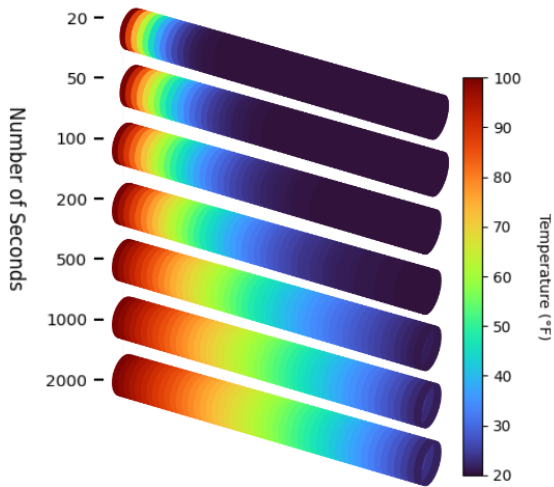
Figure 1: Time Increase as space slices are frozen
