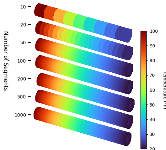
Figure 2: Space slices increase as time is frozen
