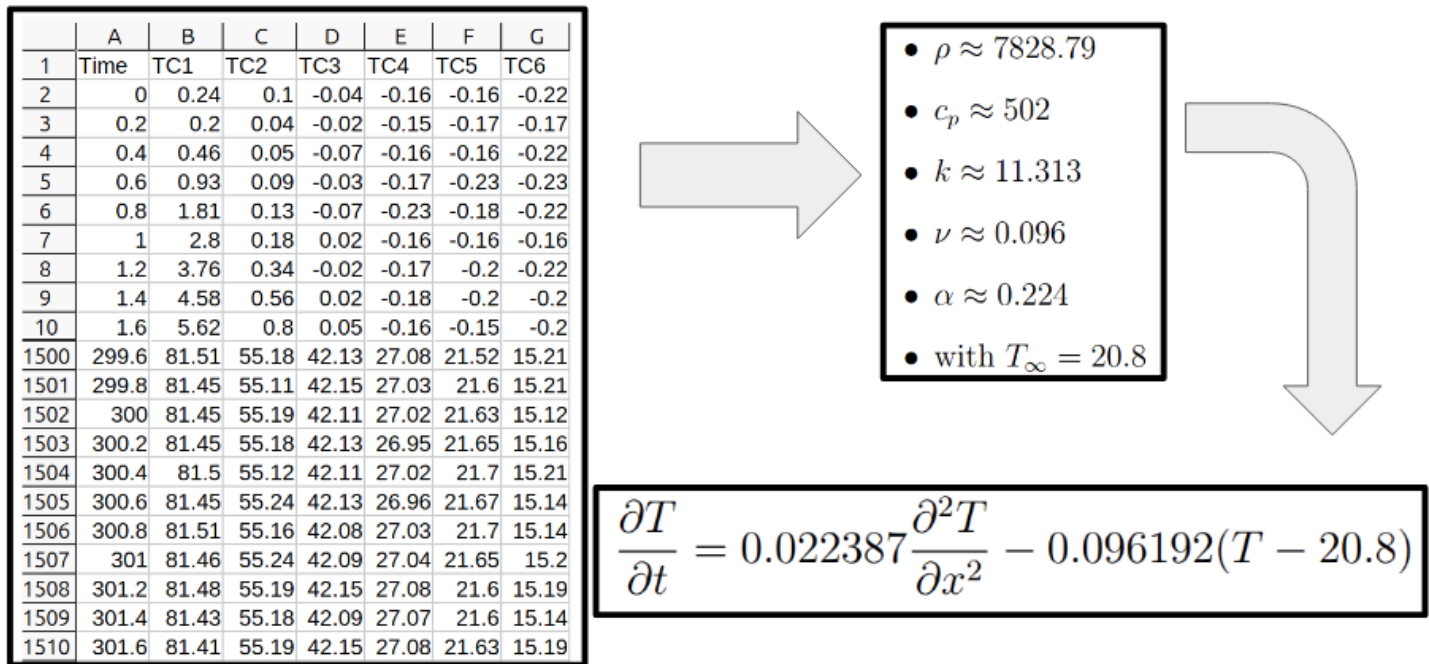
Figure 3: Data to solved parameters to completed PDE
