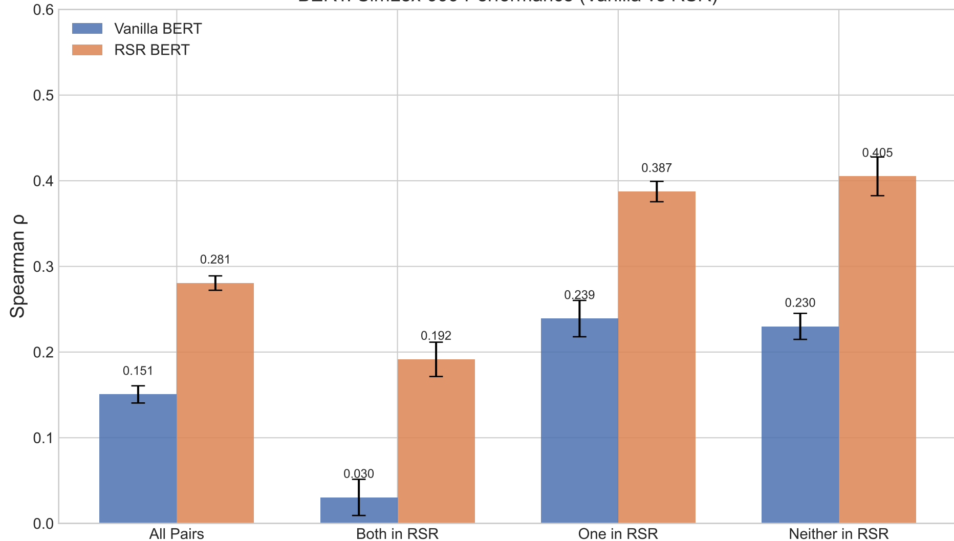
BERT: SimLex-999 Performance (Vanilla vs RSR)
