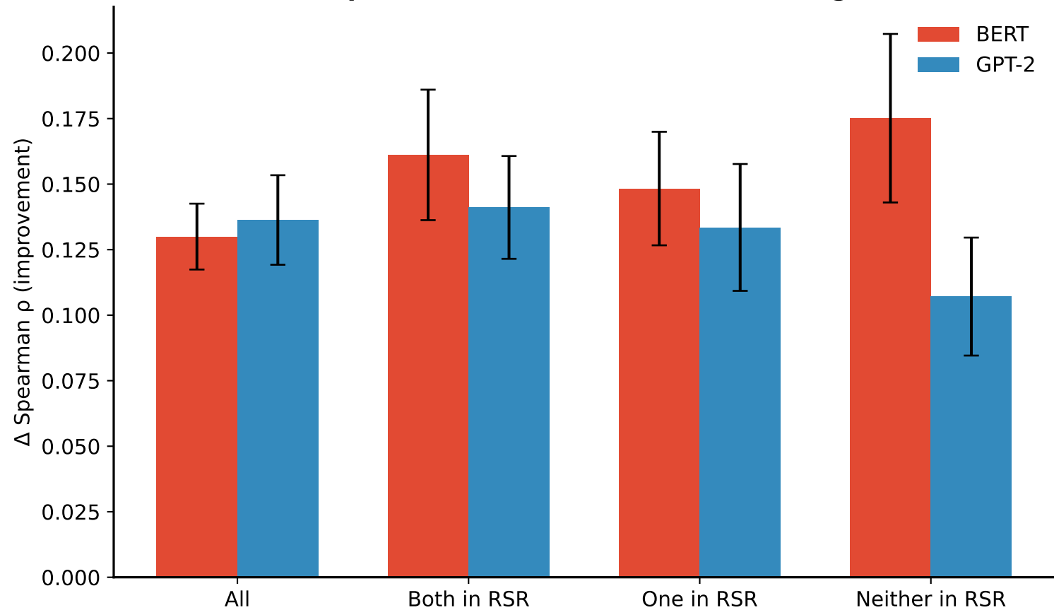
RSR Improvement Across Evaluation Categories
