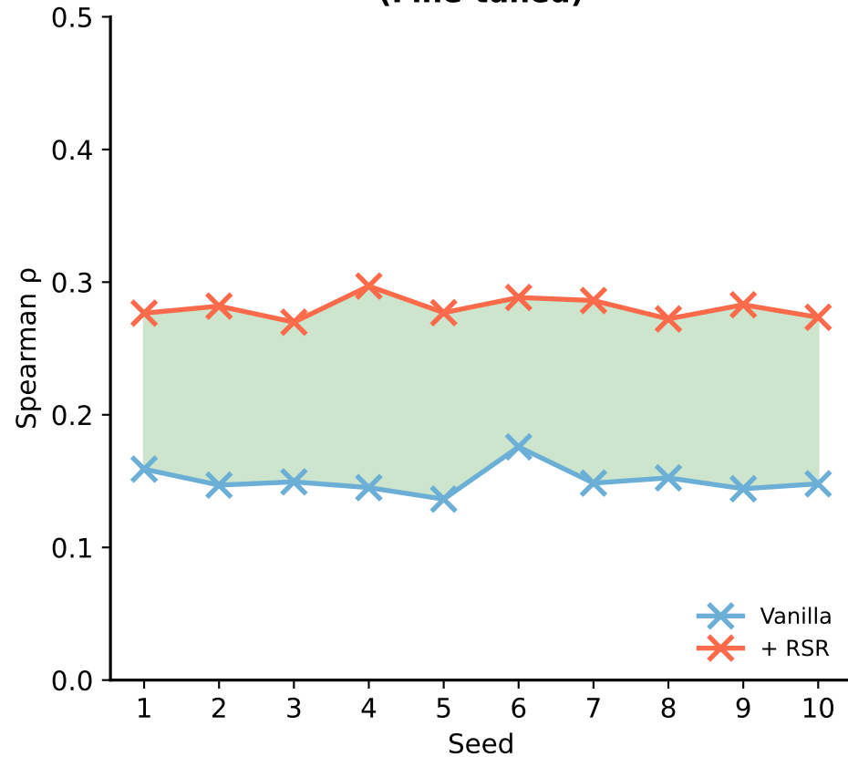
BERT (Fine-tuned)
