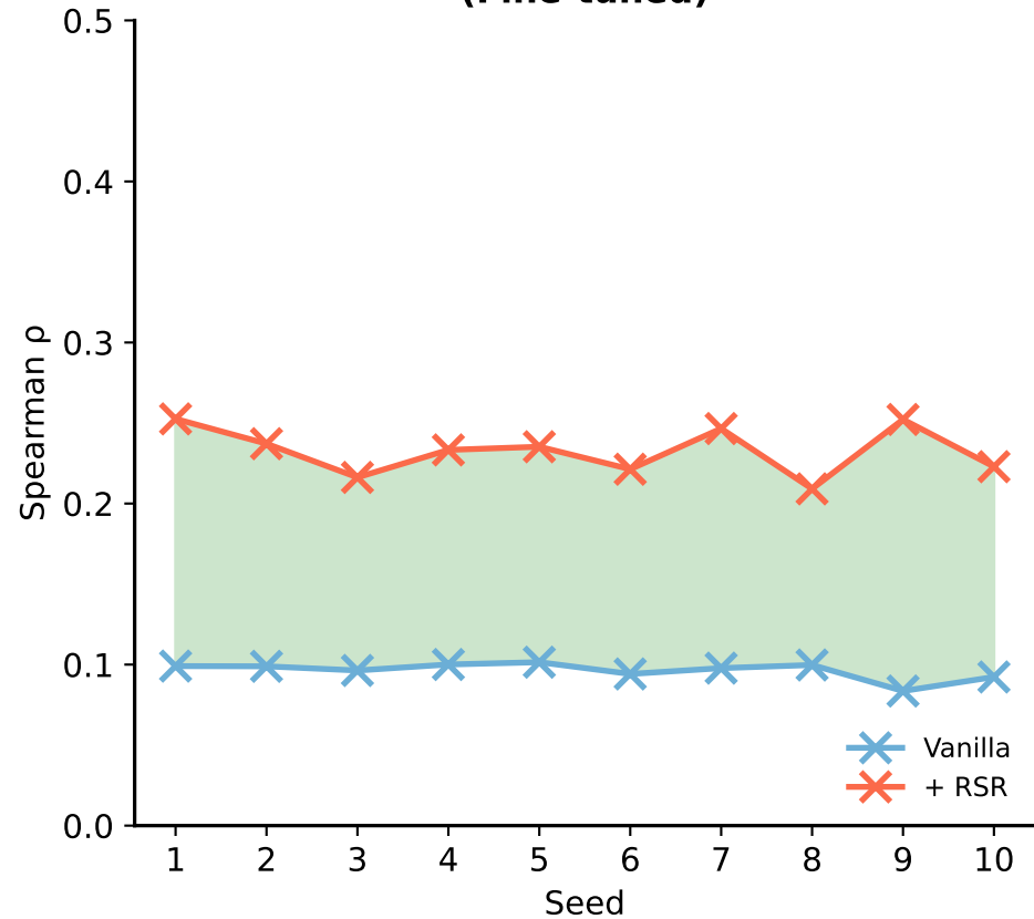
GPT-2 (Fine-tuned)
