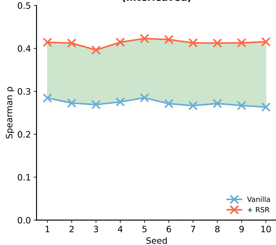
Word2Vec (Interleaved)
