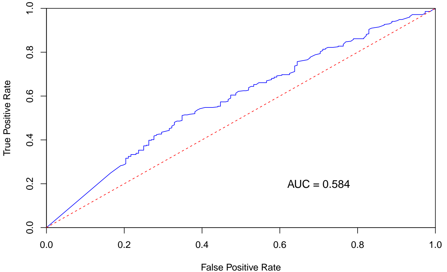
ROC Curve
