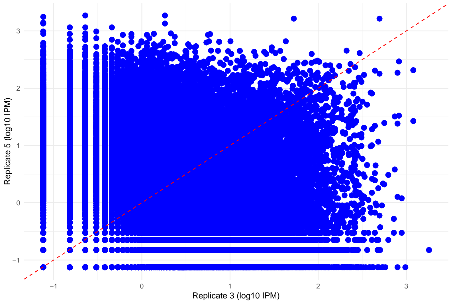
Reproducibility of Insertions from Replicates 3 and 5 (log10_IPM)
