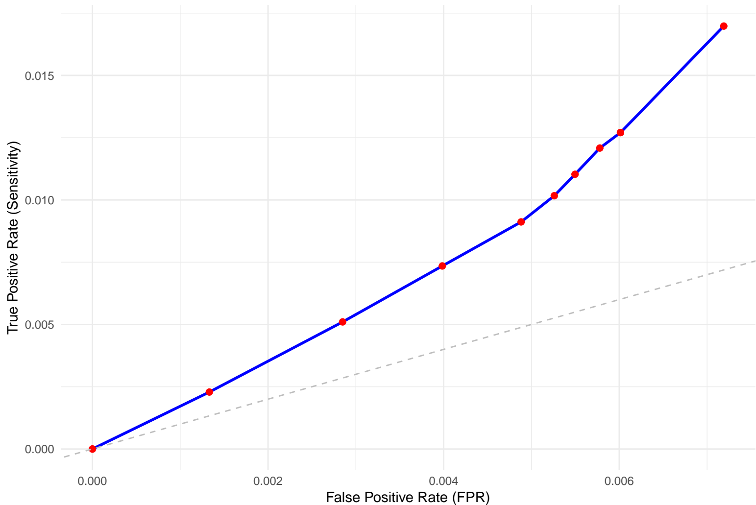
ROC Curve
