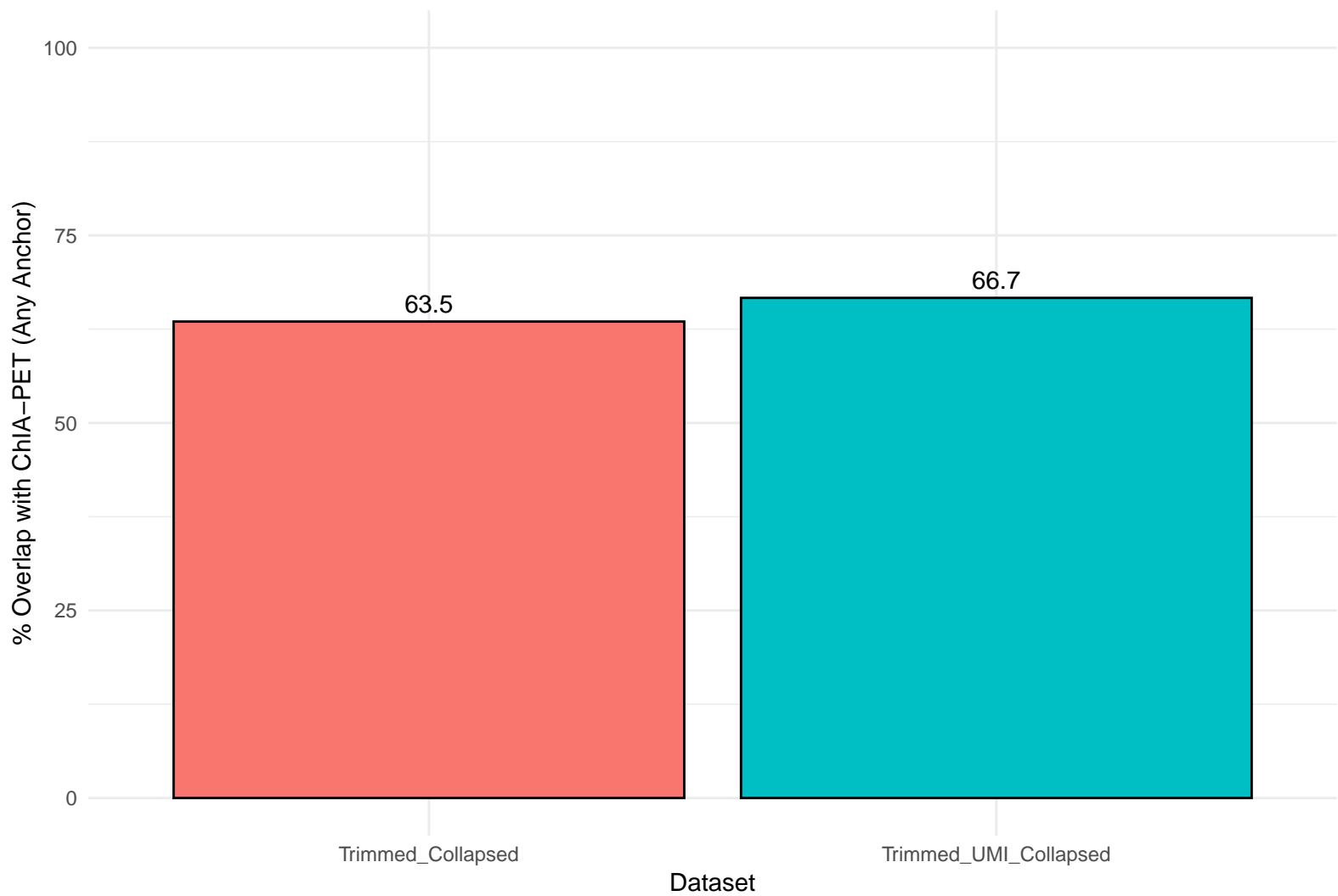
Trimmed pyCalling Cards Overlap (Collapsed qBED, Any Anchor)
