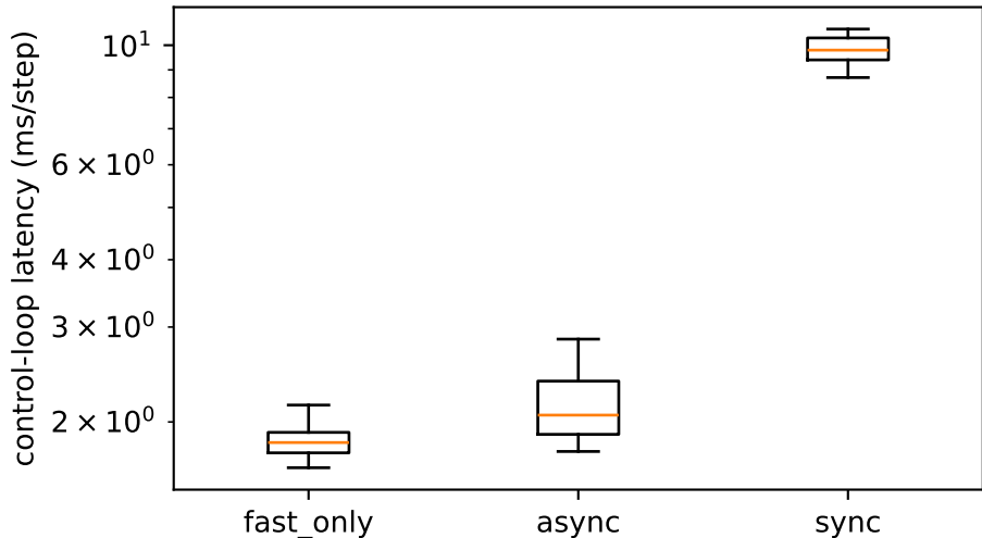
Fig D — fast/slow scheduling | async staleness=2.0 steps
