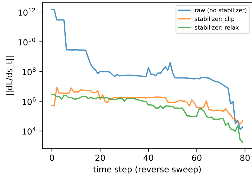
Fig E — adaptive gradient truncation
