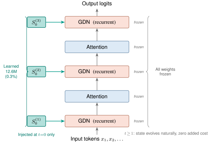
Figure 2: Computation graph for S_0 tuning. The learned initial state S_0 (teal) is injected into each recurrent layer before the first token. After t=1 , it is absorbed into the running state and adds zero computational overhead. All model weights remain frozen.
