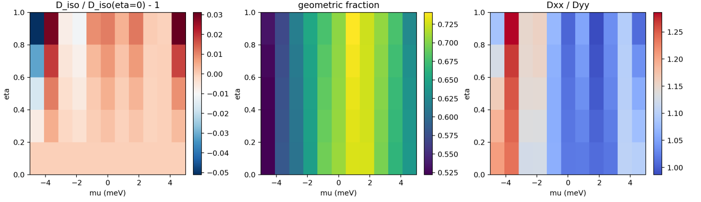
FIG. 3. Dense \mu - \eta response map in the fixed- \Delta_0 normalization. Compared with Fig. 2, the normalized response is strongly suppressed and changes sign in parts of the scan.
