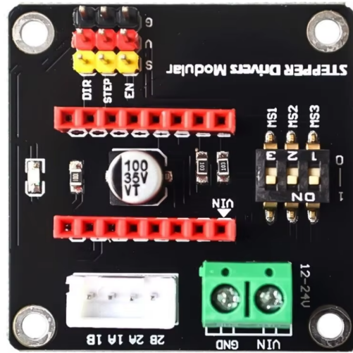
Figure 4.1: Driver expansion board
