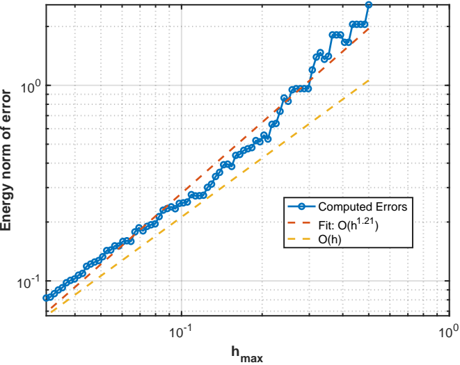
Error vs. Mesh Size
