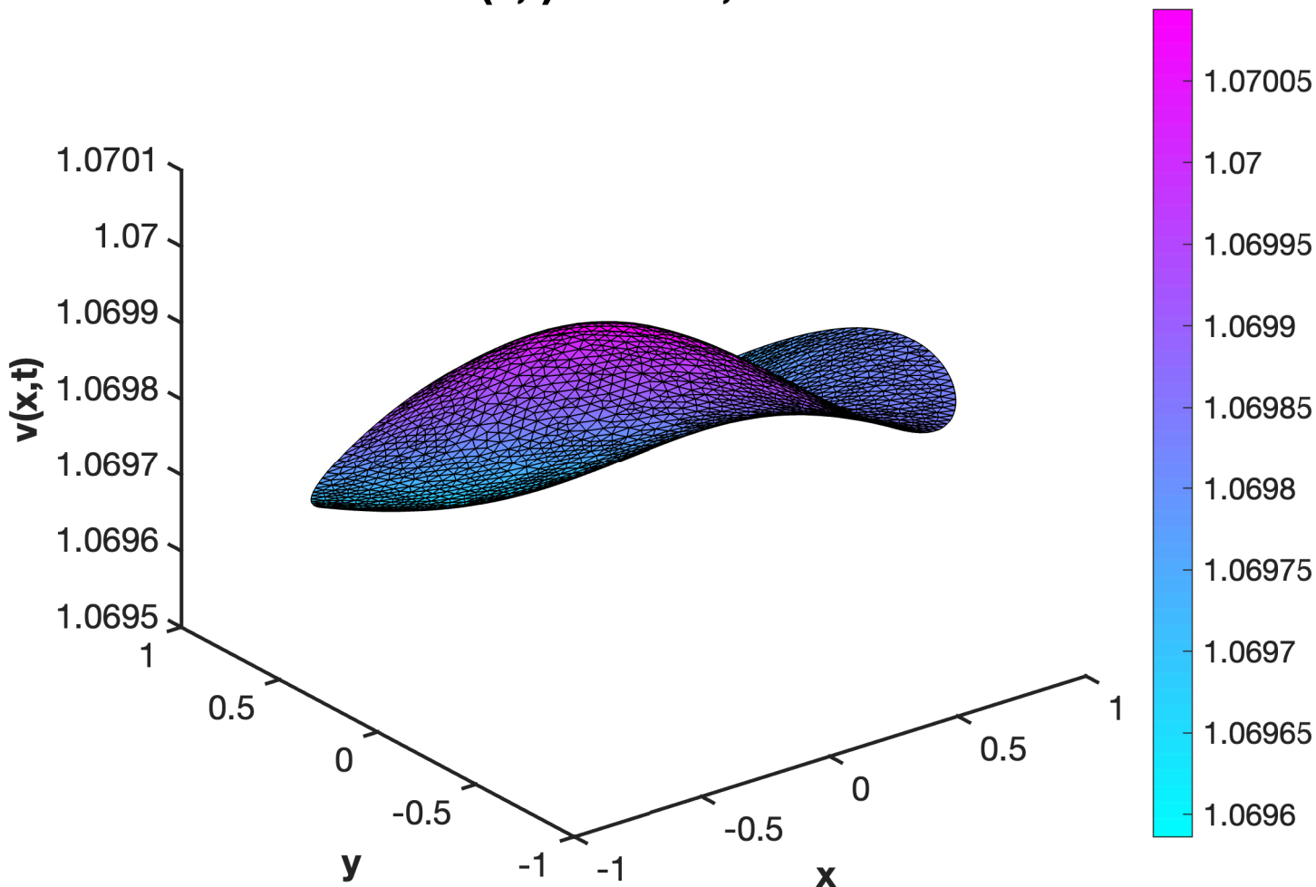
Solution v(x,t) at T = 2 , h_{\max} = 0.05
