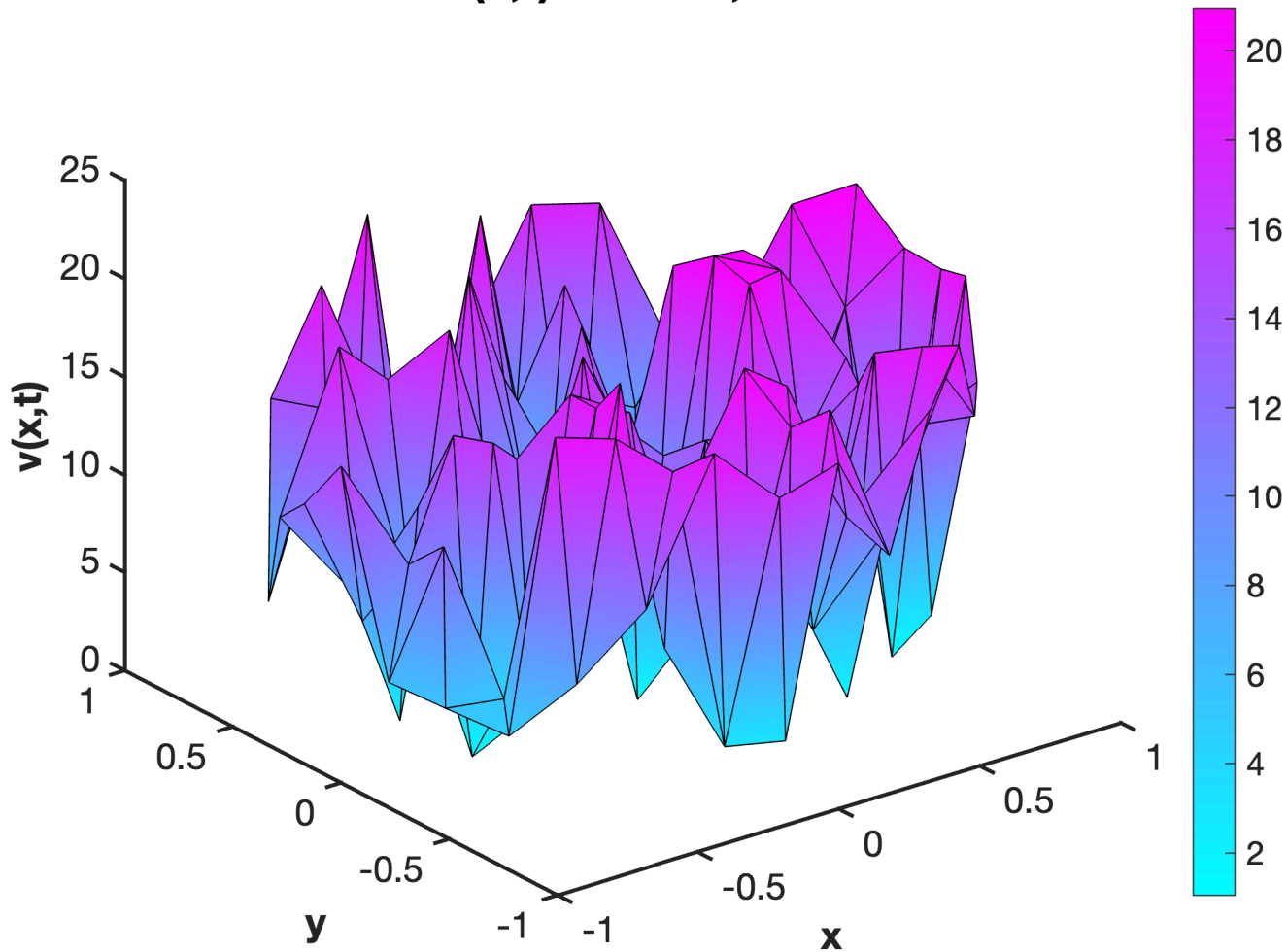
Solution v(x,t) at T = 0 , h_{\max} = 0.2
