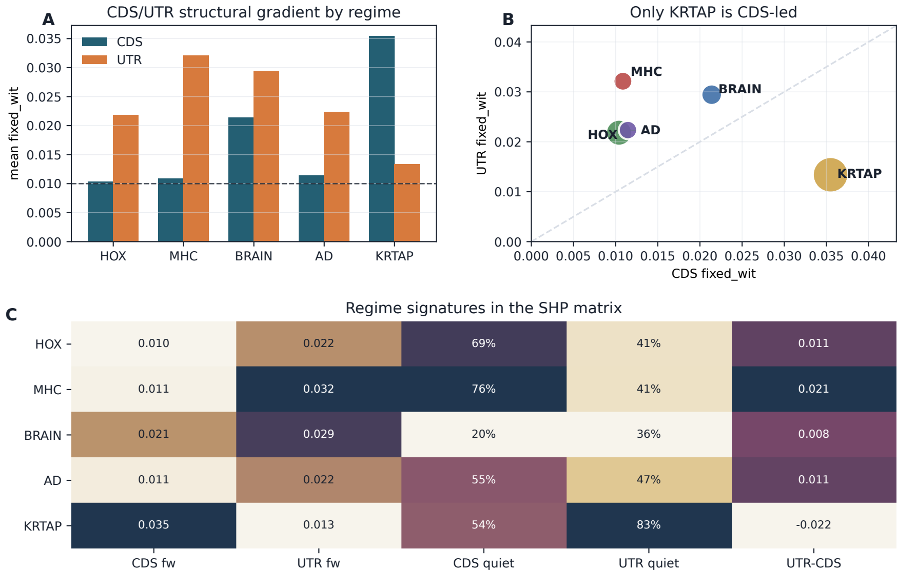
Figure 3. Biological regimes occupy distinct CDS/UTR structural states
