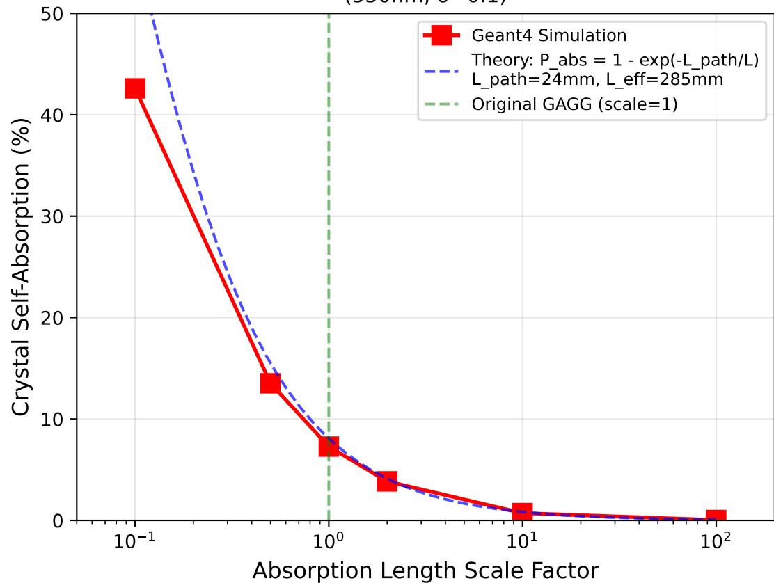
Self-Absorption vs Absorption Length Scale (550nm, \sigma=0.1 )
