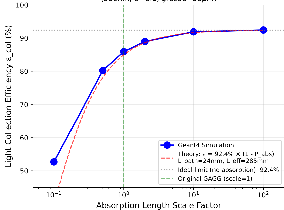
\epsilon_{\text{col}} vs Absorption Length Scale (550nm, \sigma=0.1 , grease= 50\mu\text{m} )
