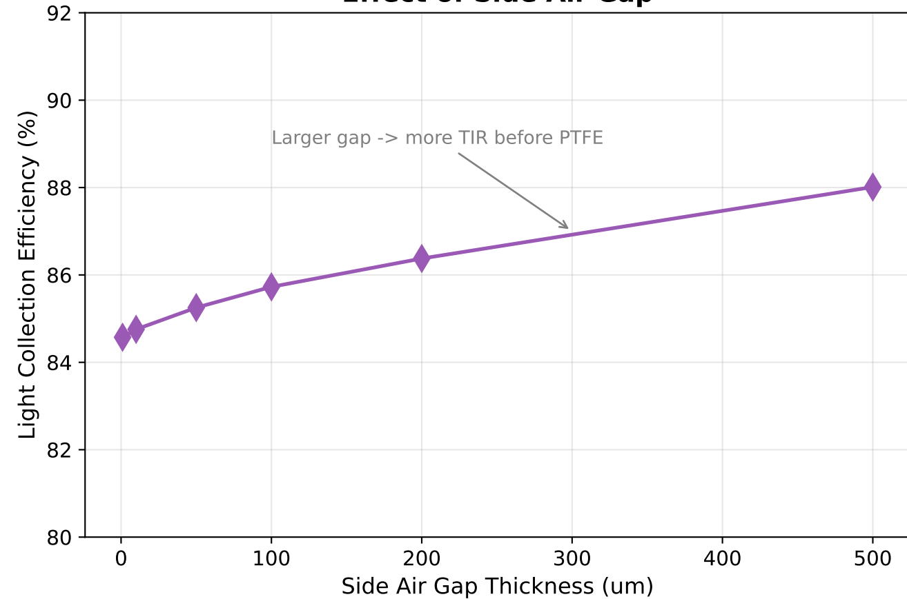
Effect of Side Air Gap
