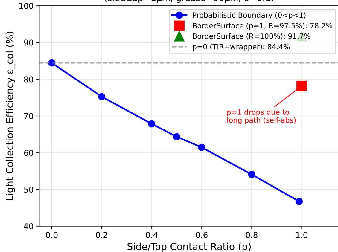
Probabilistic Boundary Method: \varepsilon_{\text{col}} vs p (sideGap=1 \mu\text{m} , grease=50 \mu\text{m} , \sigma=0.1 )
