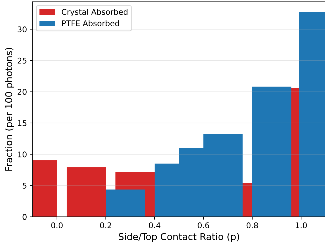
Loss Channels vs Contact Ratio
