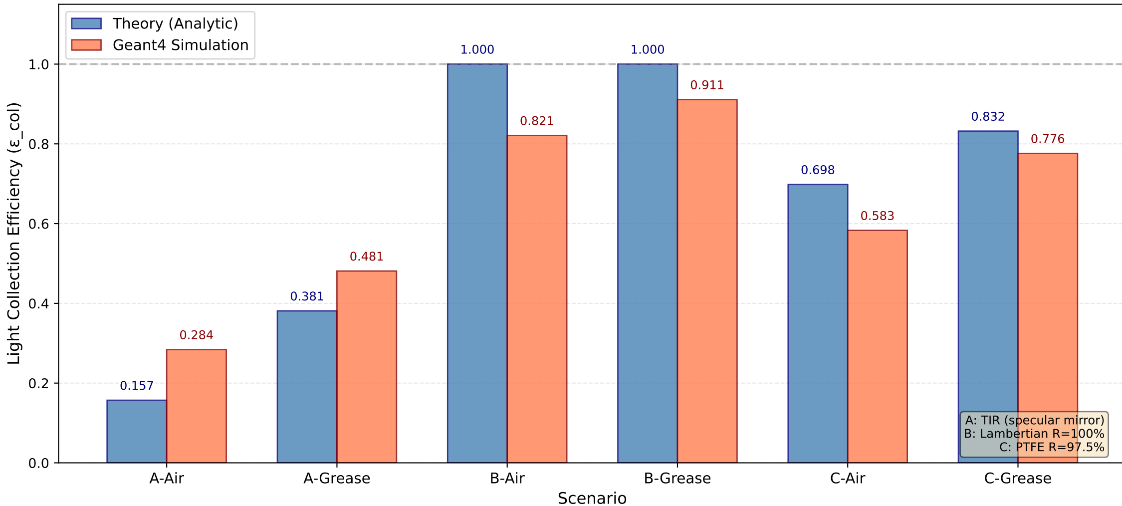
Sanity Check: Theory vs Geant4 Simulation (GAGG 5×5×5 mm 3 , 10000 photons, original absorption)
