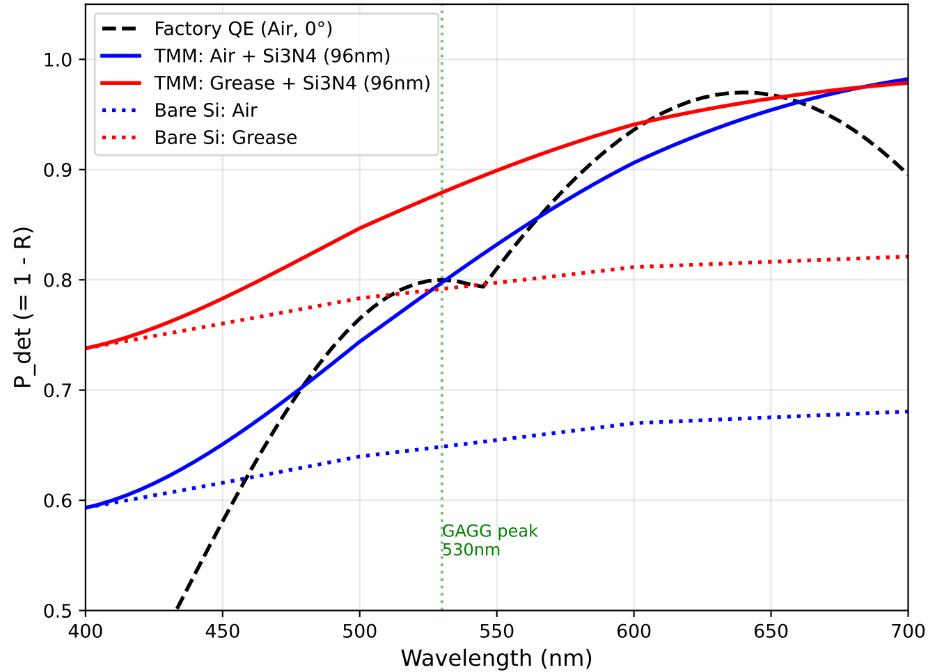
P_det(λ,θ) for Grease Incidence (Si3N4 d=96nm)
