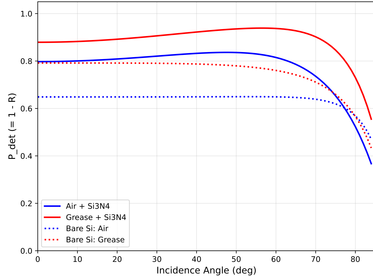
Angular Dependence @ 530nm
