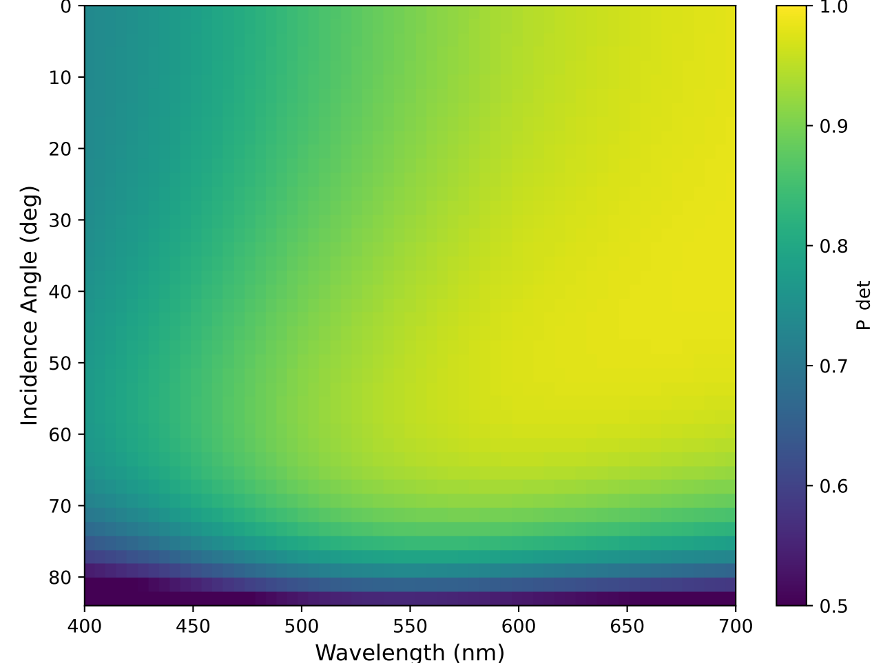
P_det(λ,θ) for Grease Incidence (Si3N4 d=96nm)
