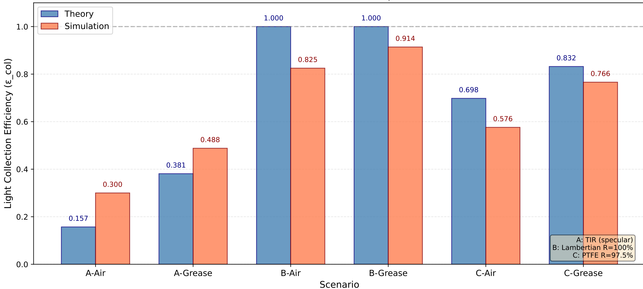
Sanity Check: Theory vs Geant4 Simulation (GAGG 5×5×5 mm 3 , 1000 photons)
