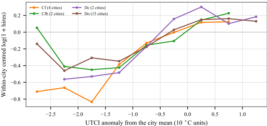
Thermal response by Trewartha climate group
