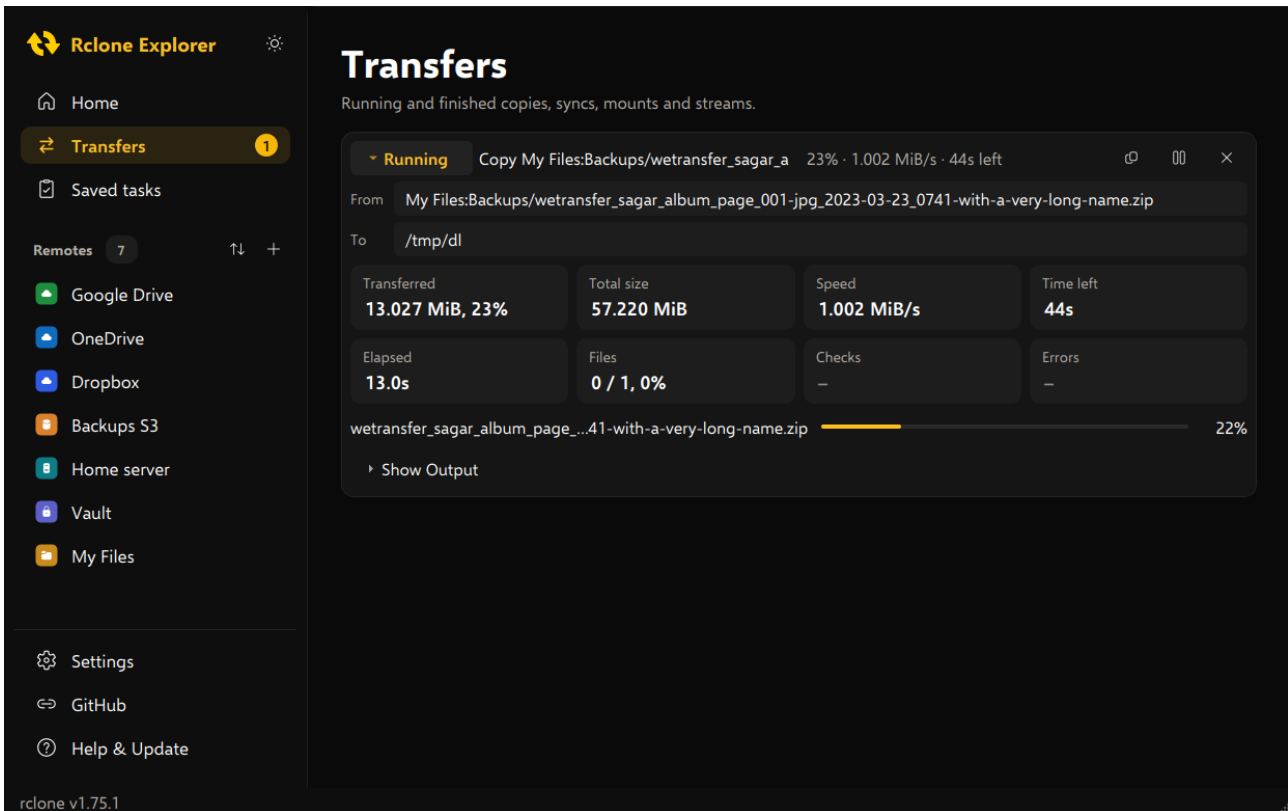
A running transfer with statistics tiles and per-file progress.
