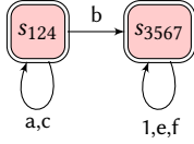
Figure 5: Automata A_1 without blue states
