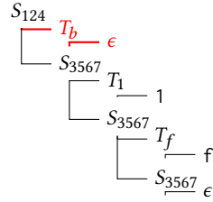
Figure 8: 1fX Parse tree.
