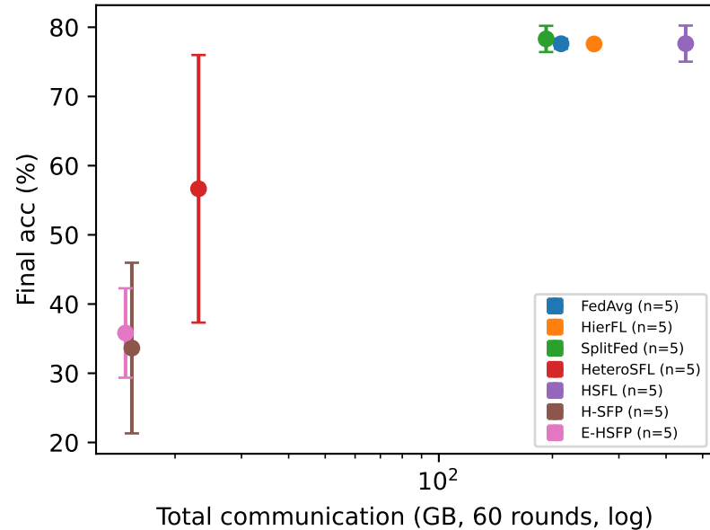
ham10000
