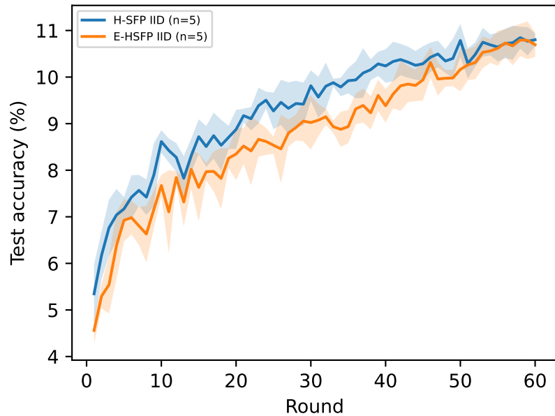
CIFAR-100
