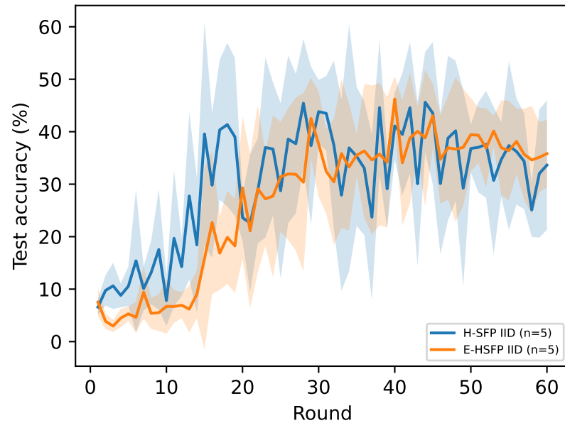
HAM10000
