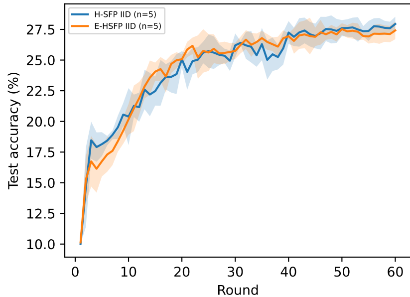
CIFAR-10
