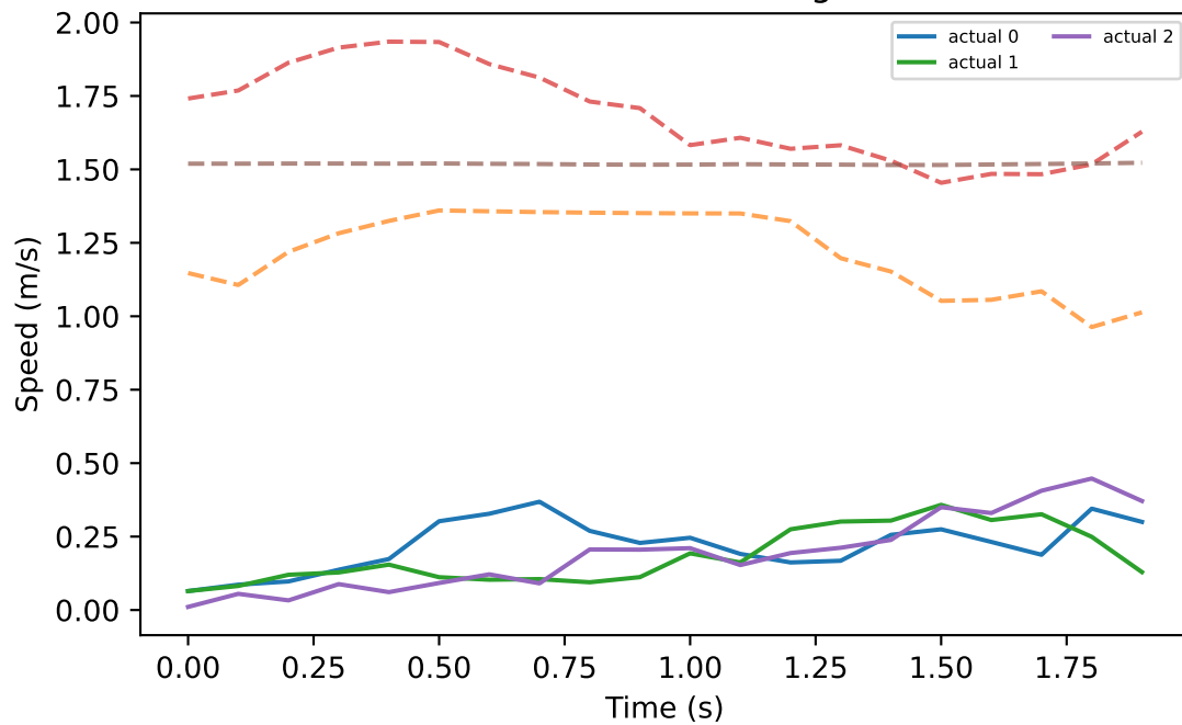
Command tracking
