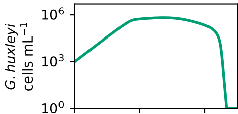
Cluster 1
