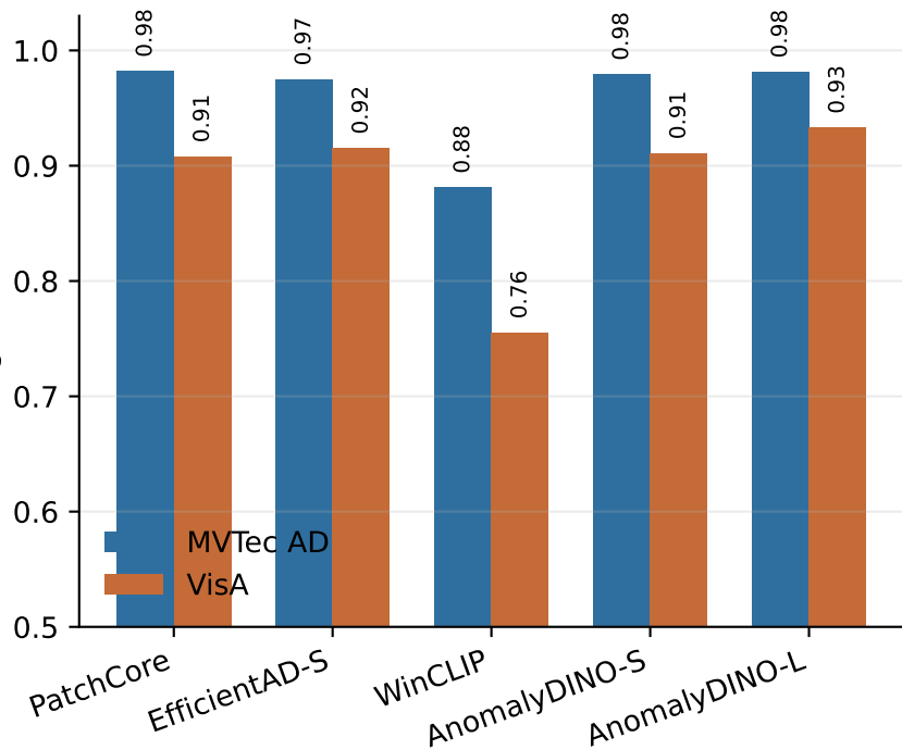
Image AUROC
