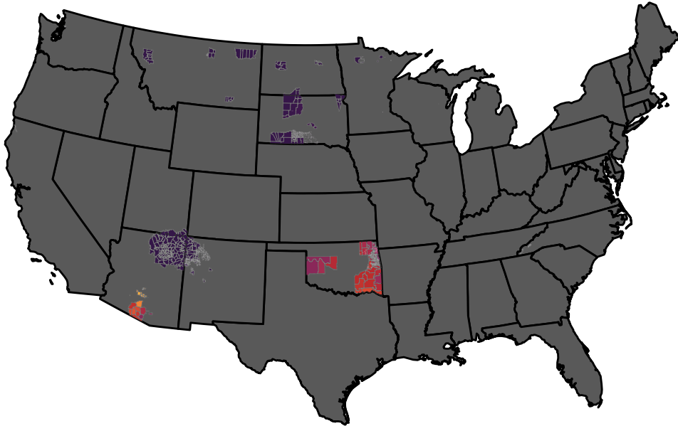
Mean annual number of dangerous hot-humid days (WBGT > 28°C) during 2016–2020 0 20 40 60 80
