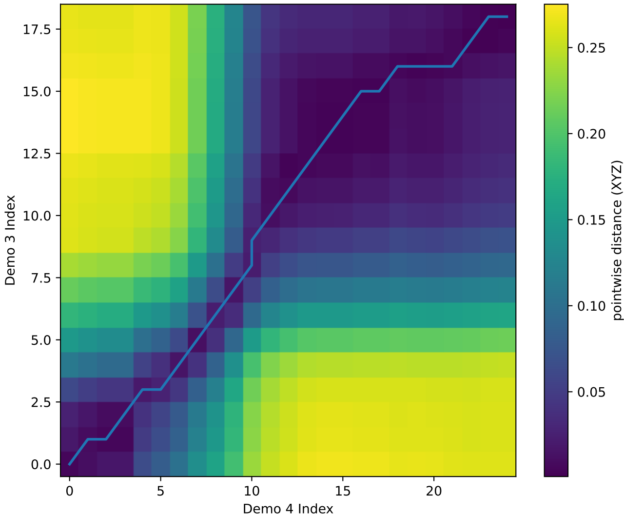
Traj3 vs Traj4: DTW cost + path (factor=8)
