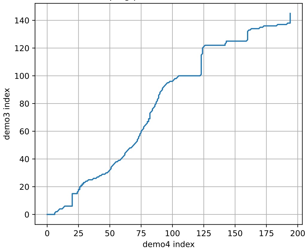
DTW warping path: demo3 \rightarrow demo4 (XYZ)
