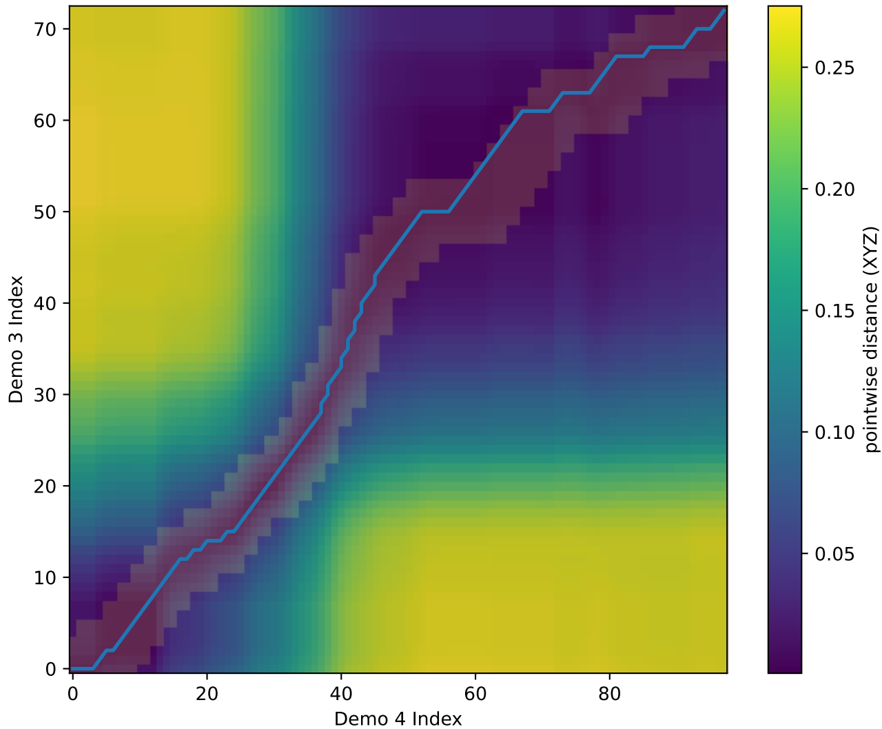
Traj3 vs Traj4: DTW cost + path (factor=2)
