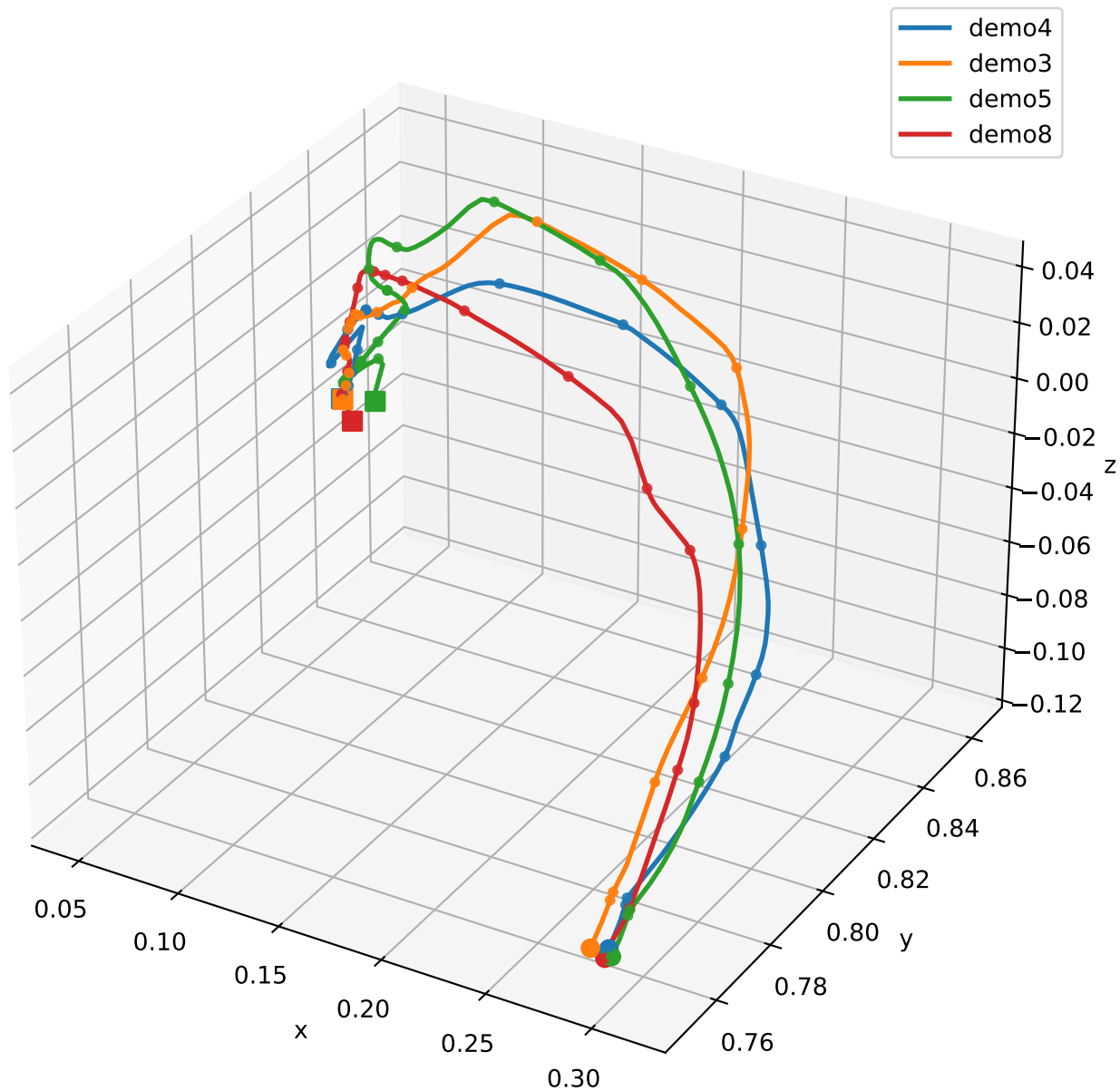
Multiscale DTW aligned to demo4 timeline (XYZ)
