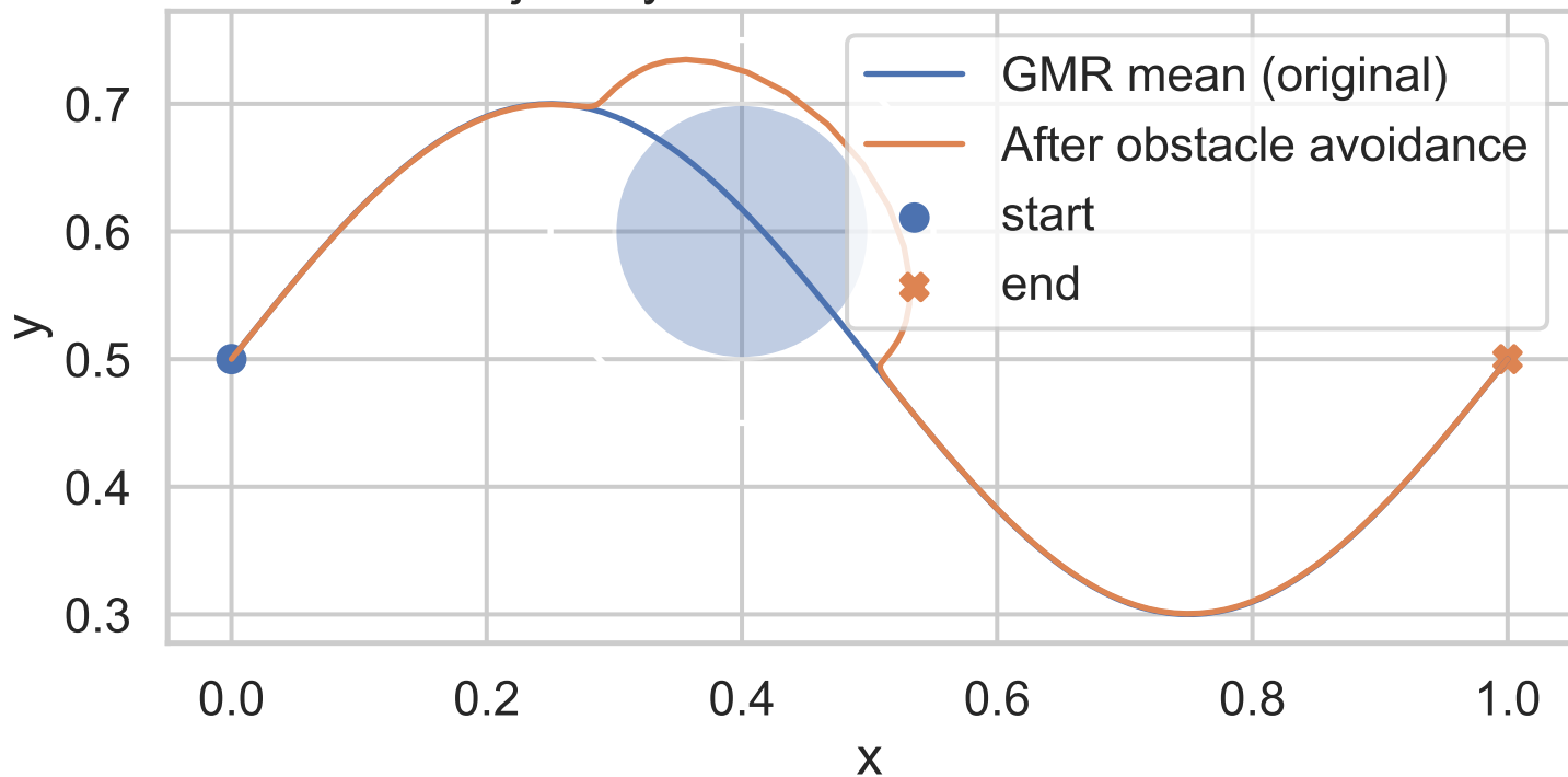
GMR trajectory with circular obstacle avoidance
