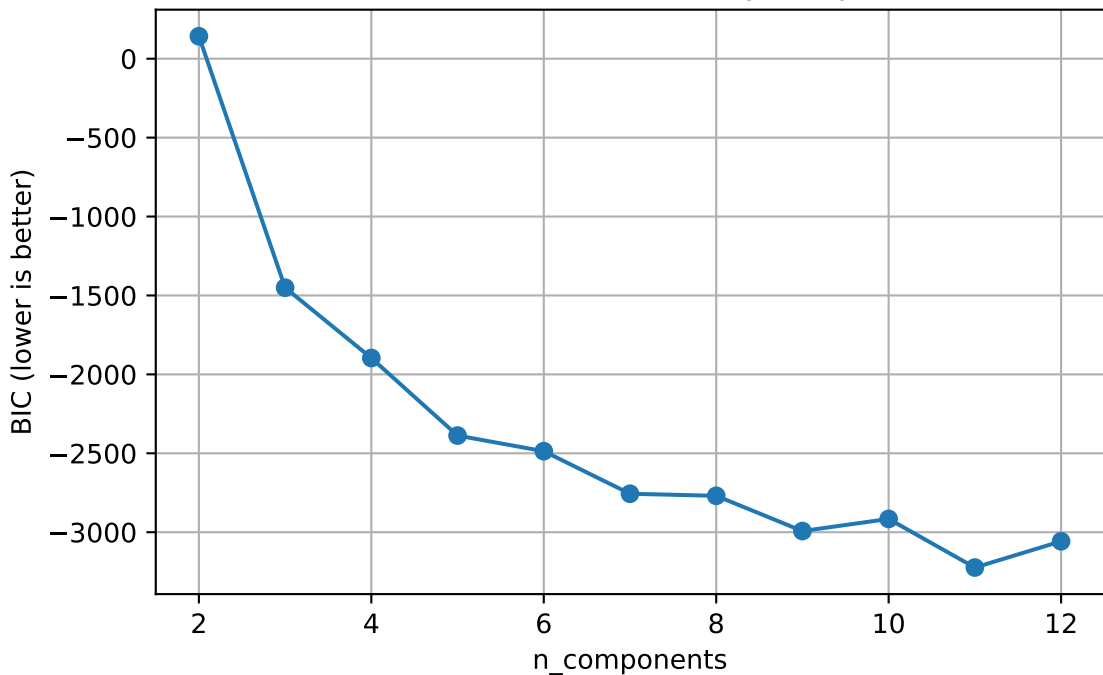
GMM model selection by BIC.pdf
