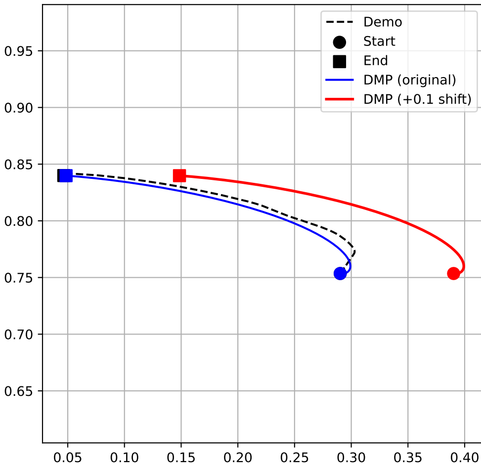
DMP Generalization Test: +0.1 \times \text{Offset}
