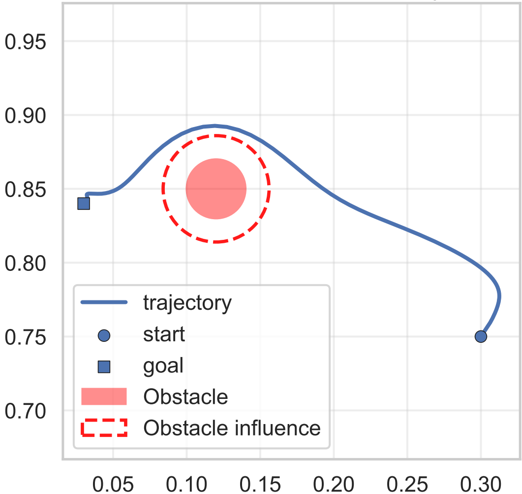
With obstacle avoidance – XY projection
