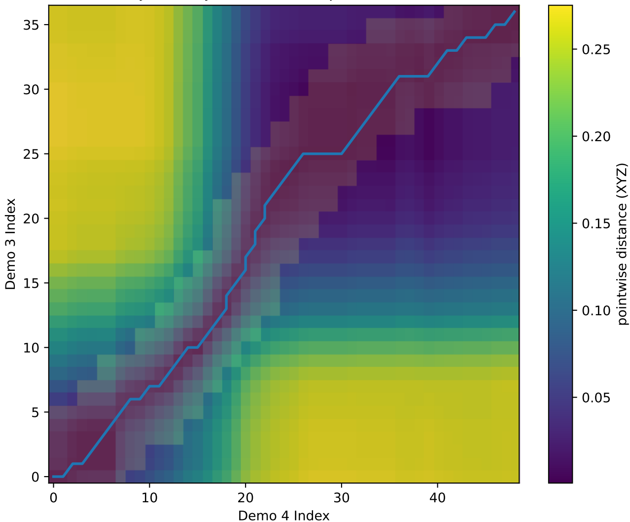
Traj3 vs Traj4: DTW cost + path (factor=4)
