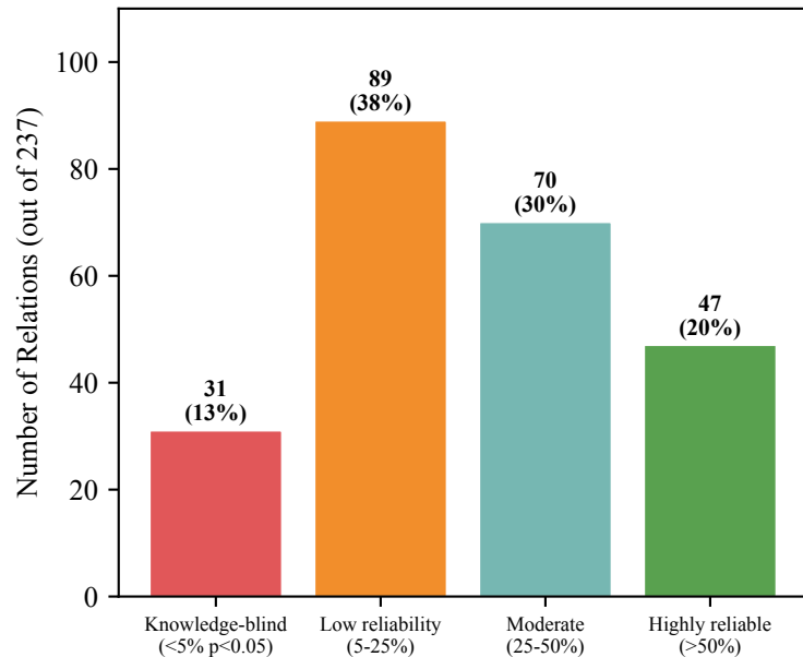
FB15k-237: Per-Relation Reliability Distribution (RotatE)
