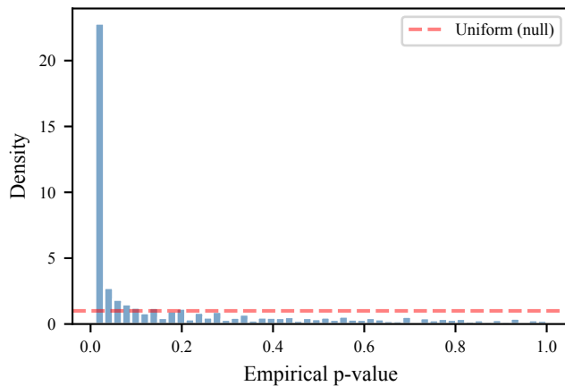
ConvE ( \hat{\pi}_0 = 0.321 )
