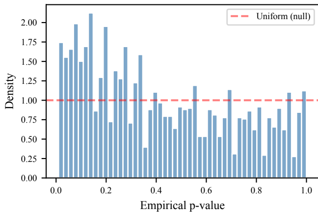
Complex ( \hat{\pi}_0 = 0.754 )
