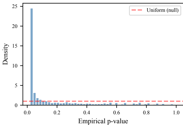
Complex ( \hat{\pi}_0 = 0.754 )
