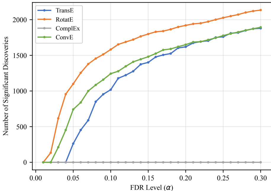
Figure 4: Statistical Power vs. FDR Level
