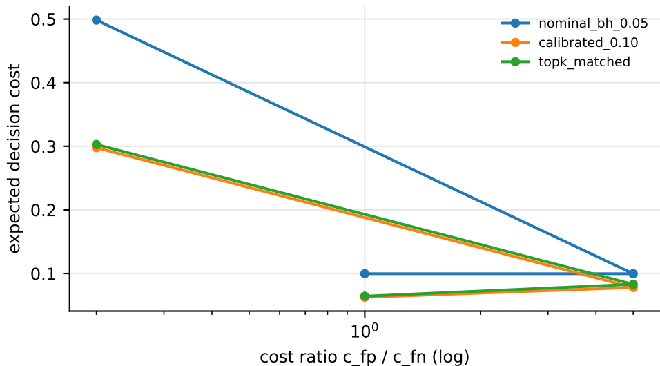
Decision cost vs cost asymmetry
