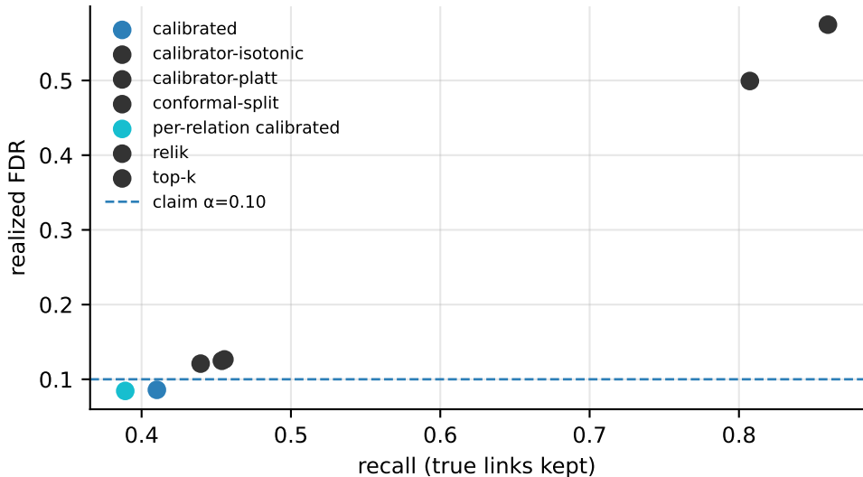
Screening methods: error vs recall
