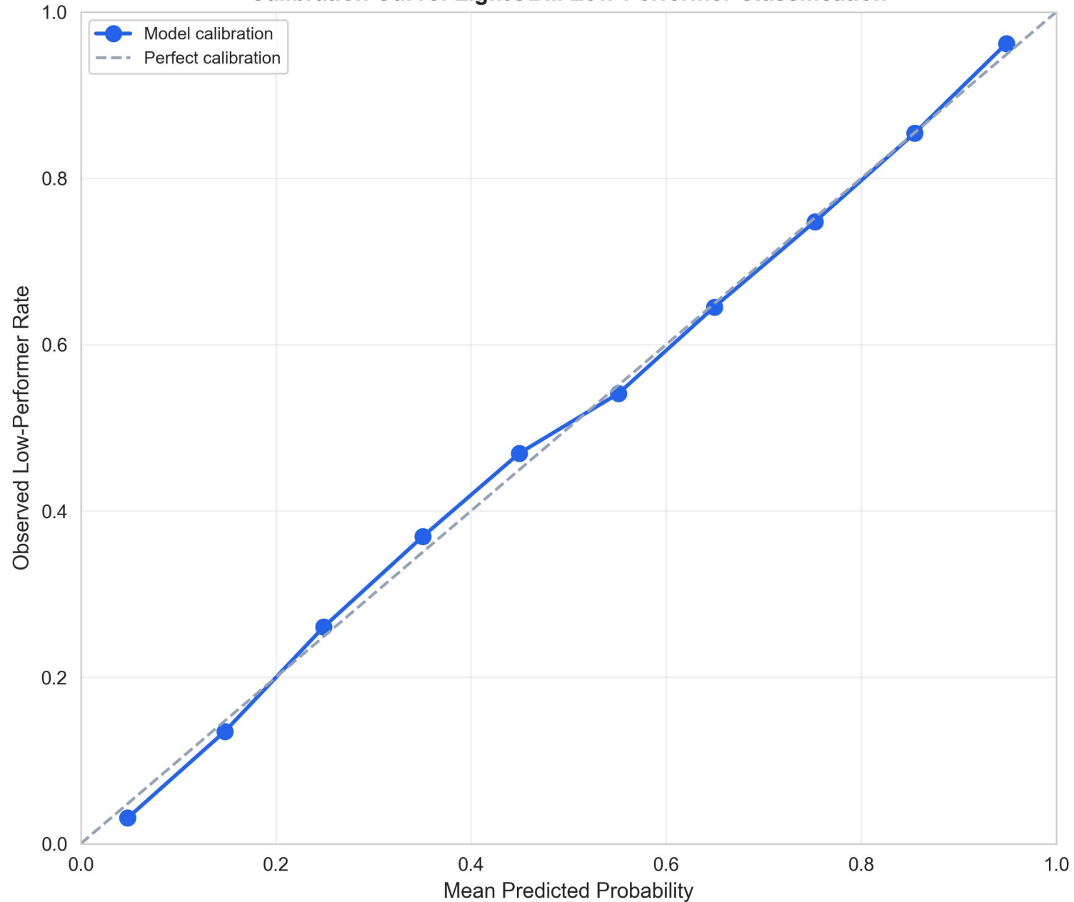
Calibration Curve: LightGBM Low-Performer Classification
