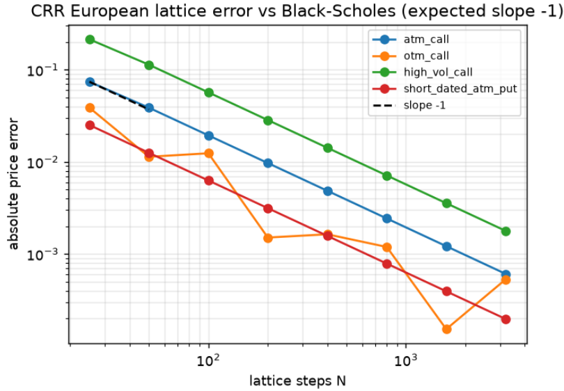
Figure 1: CRR lattice error against N on log-log axes, the source of Table 2. Generated figure, committed at experiments/pricing_validation/results/lattice\_convergence.png .
