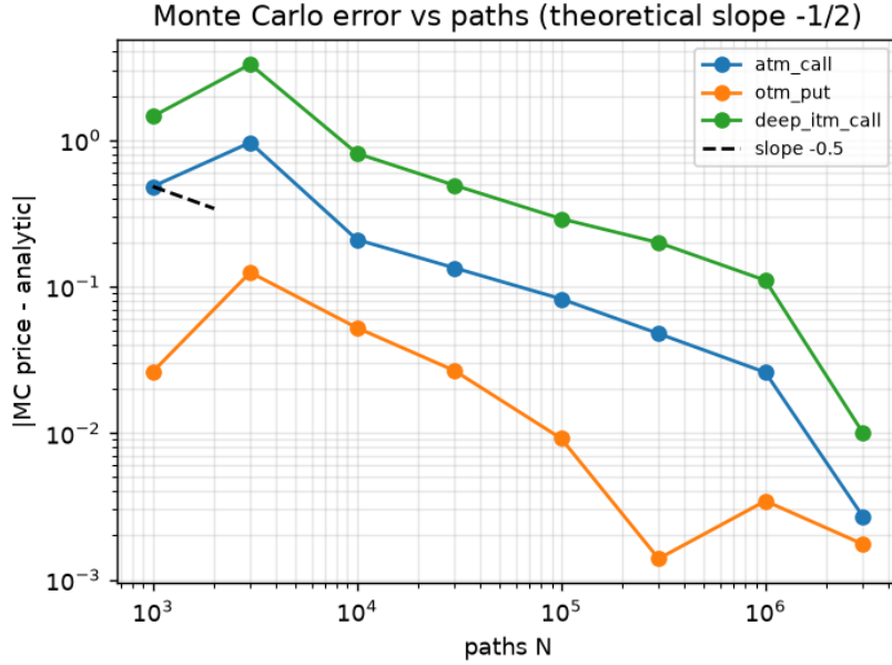
Figure 2: Fitted slope of \log|\text{error}| on \log N against the theoretical -0.5 , the source of the figures in Section 5. Generated figure, committed at experiments/monte_carlo_convergence/results/convergence\_slope.png .
