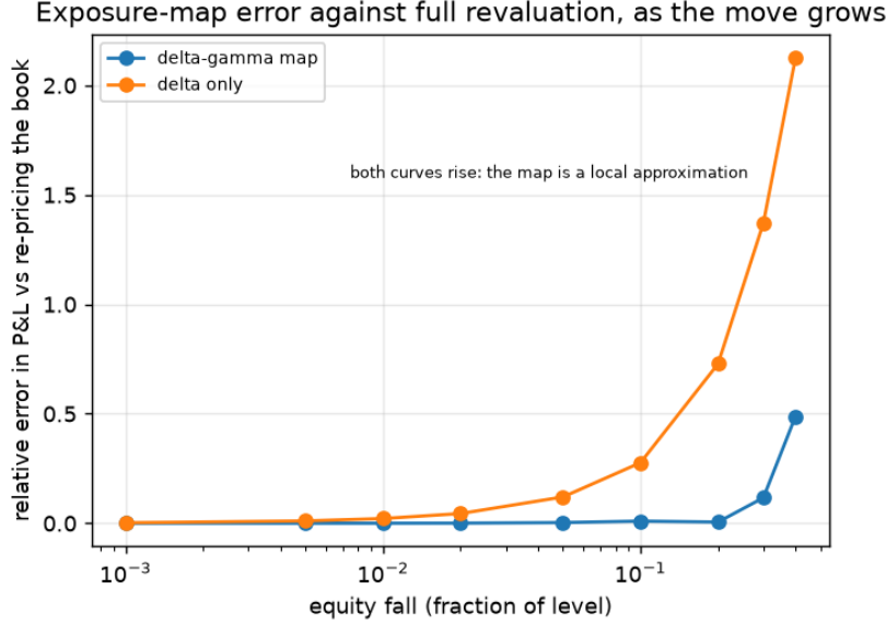
Figure 4: Relative P&L error of the delta–gamma and delta-only maps against a full Black–Scholes revaluation, the source of Table 11; the non-monotone segment is visible. Generated figure, committed at experiments/stress\_testing/results/linearisation\_error.png .
