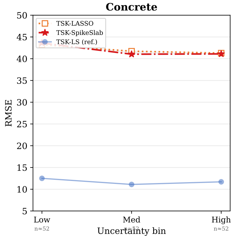
Fig. 5: Mechanism: RMSE by uncertainty bin
