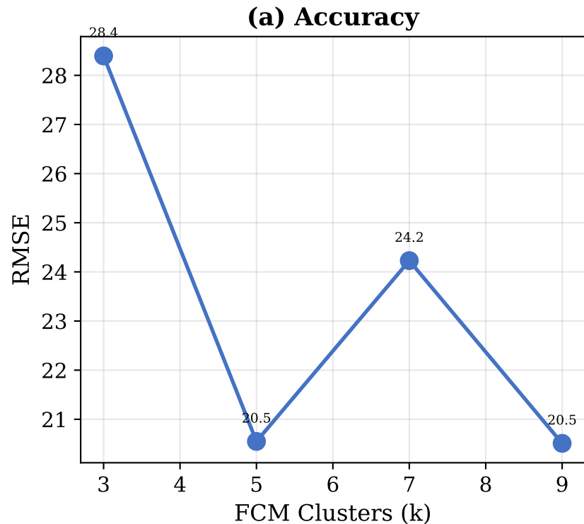
Fig. 4. FCM cluster count sensitivity
