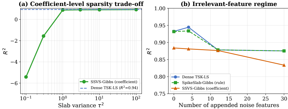
Sparsity boundary under correct fuzzy c-means
