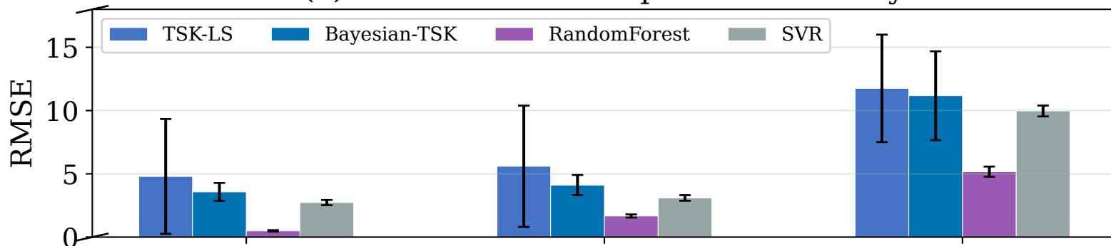
(a) Methods with competitive accuracy
