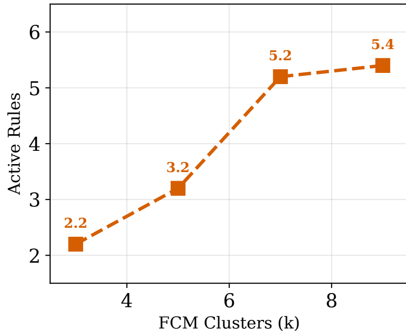
(b) Sparsity
