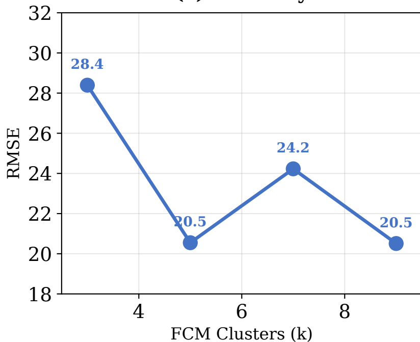
(a) Accuracy
