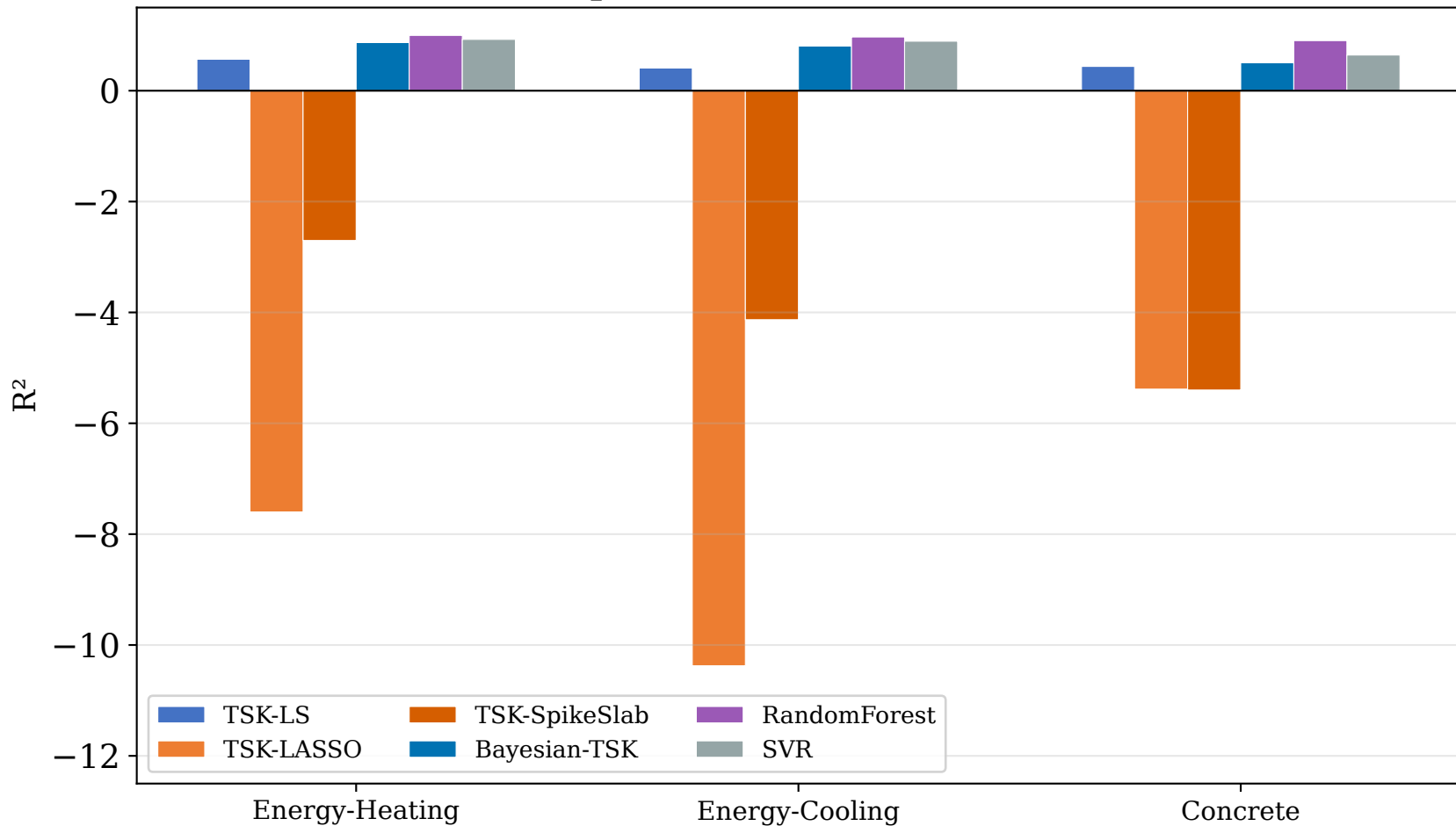
Predictive performance ( R^2 ) across datasets
