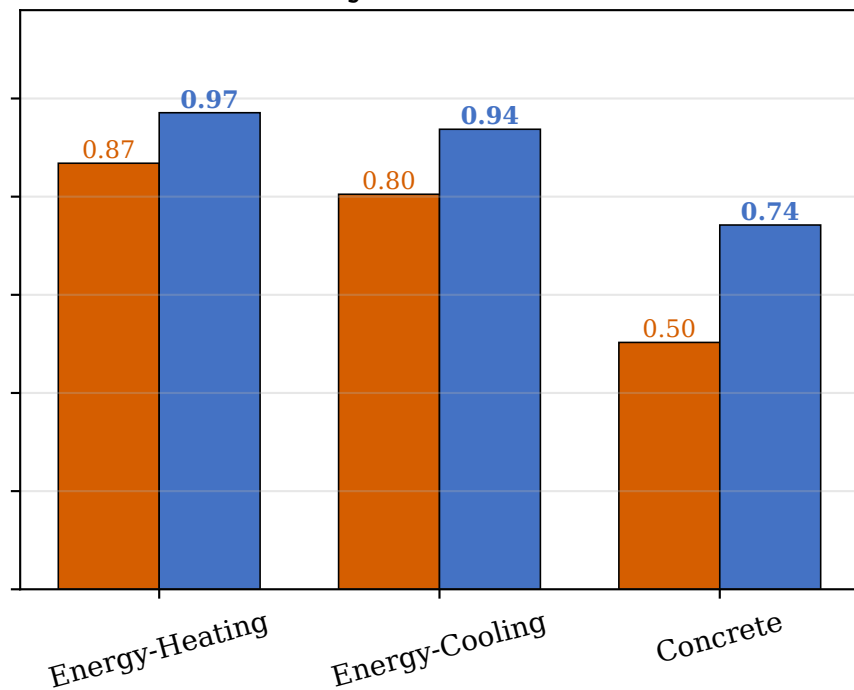
Bayesian-TSK
