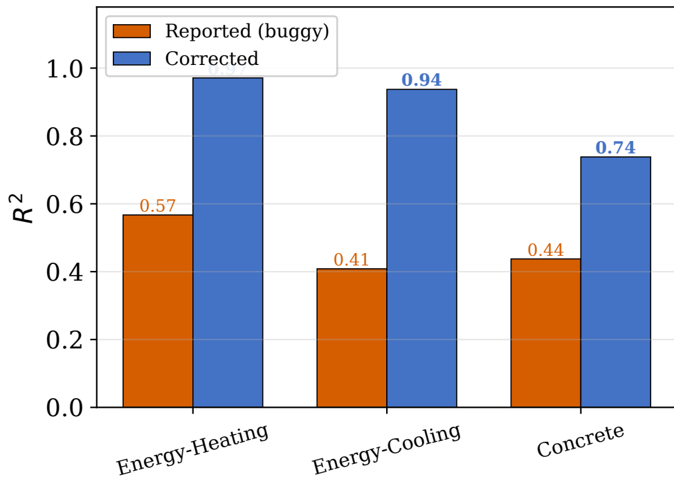
TSK-LS
