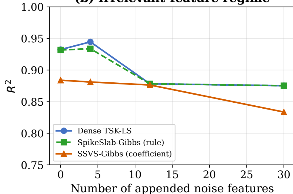
(b) Irrelevant-feature regime
