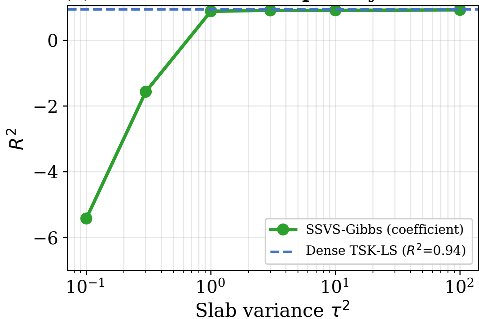
(a) Coefficient-level sparsity trade-off
