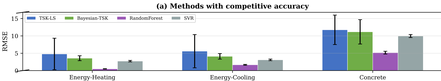
Fig. 1. Prediction accuracy (RMSE) across methods and datasets
